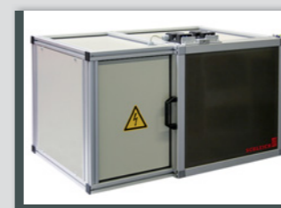
Test cage for material testing up to 40KV
