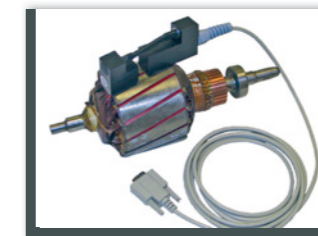
Winding detection at a rotor with flexible induction test probe
